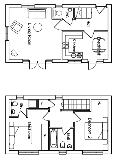
GROUND FLOOR PLAN FIRST FLOOR PLAN PLOT 15. 78 sq.m.
