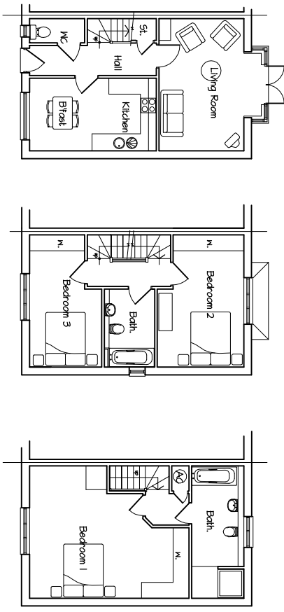
GROUND FLOOR PLAN FIRST FLOOR PLAN PLOTS 1 & 2. 122 sq.m.
